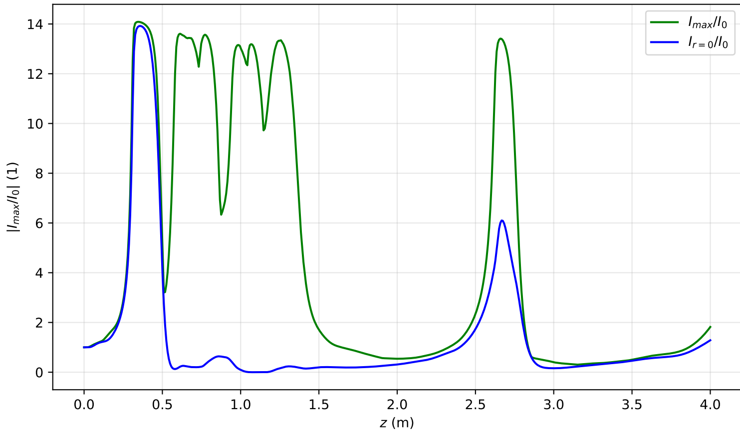
I_{max}(x=0, y=0, z)/I_0 , Pin=7.9Pcr, noisy input, artificial time
